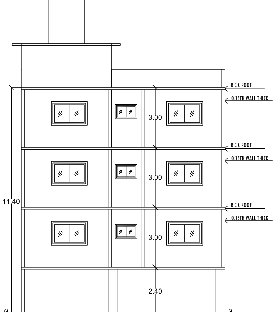
SECTION X-X
